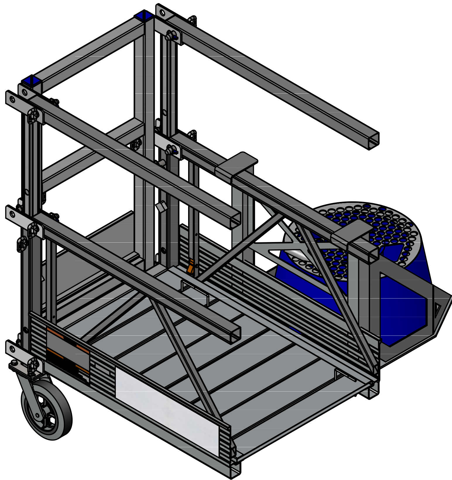
Passive Wire Winder installed on 3933-200 (Wire Winder Hanger):
