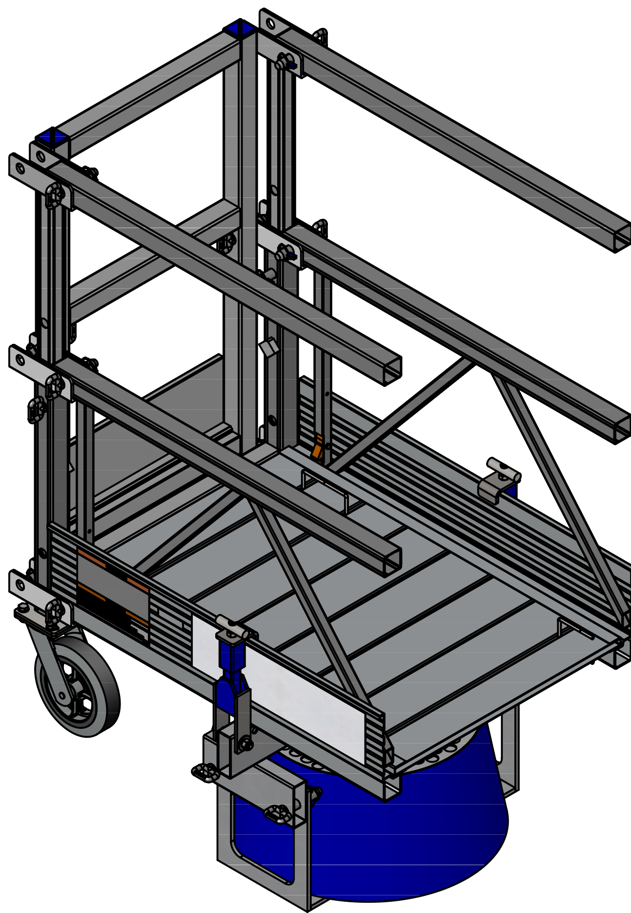
Passive Wire Winder installed on 3471-3 (Wire Winder Mounting Bracket):
