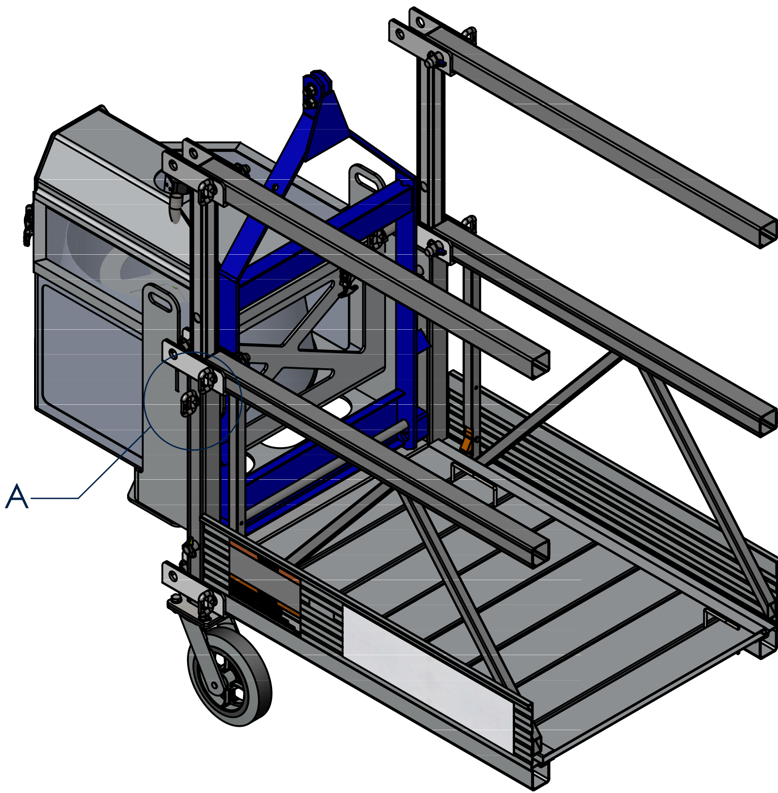
Platform View: High-Capacity Passive Wire Winder installed on Sky Stage Ultra with End Stirrup (360150):
