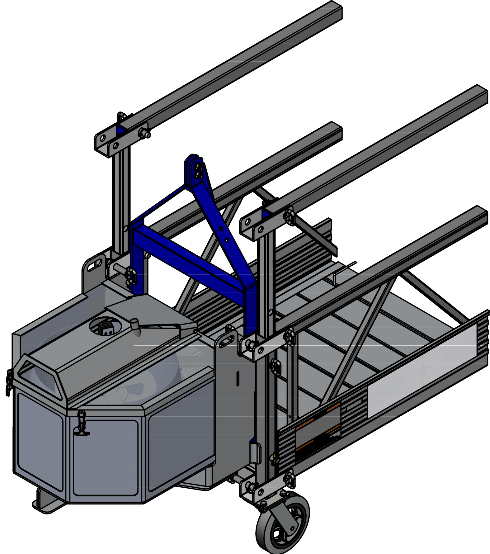
End View: High-Capacity Passive Wire Winder installed on Sky Stage Ultra with End Stirrup (360150):
