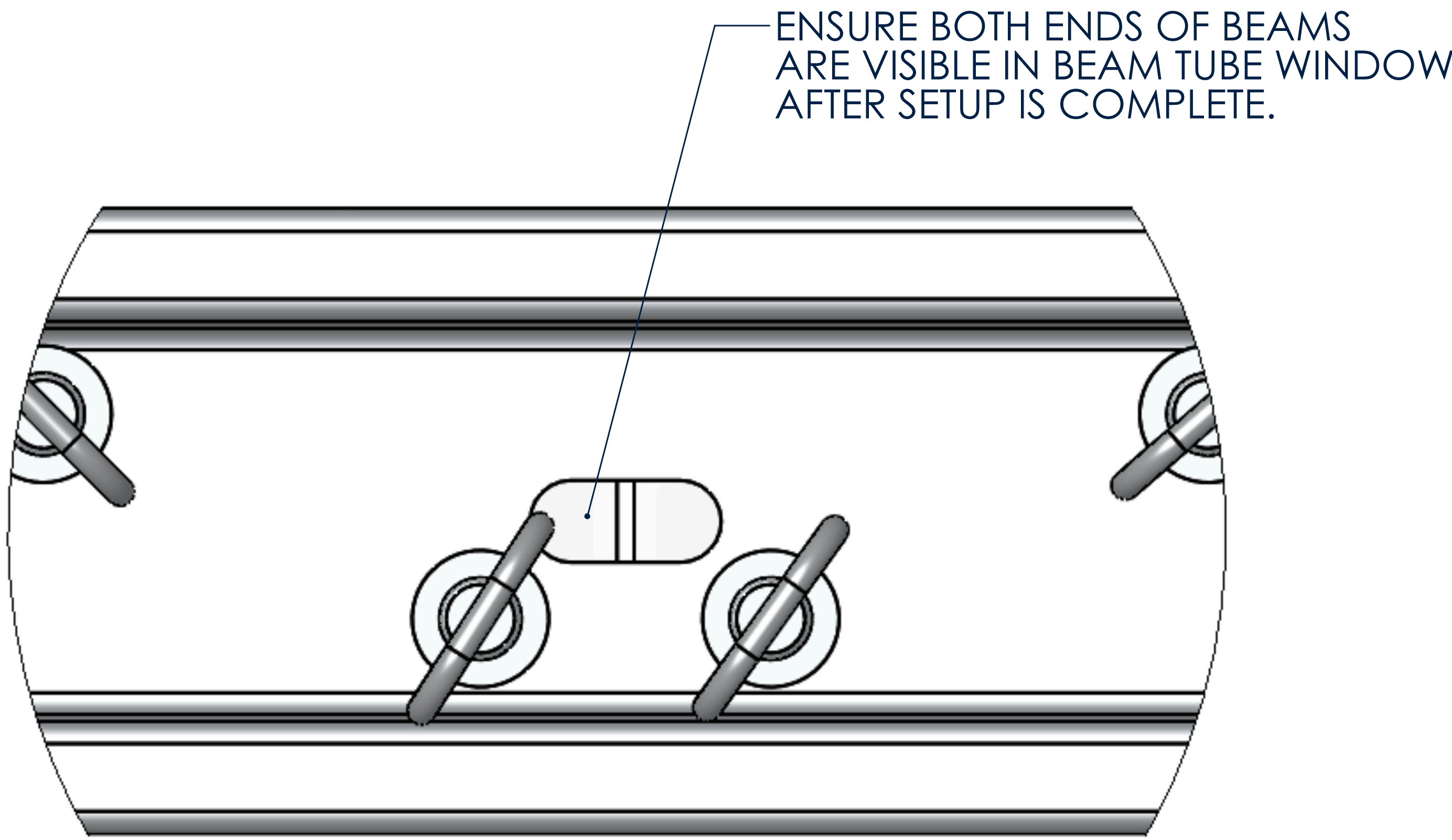
DETAIL A SCALE 1 : 2
